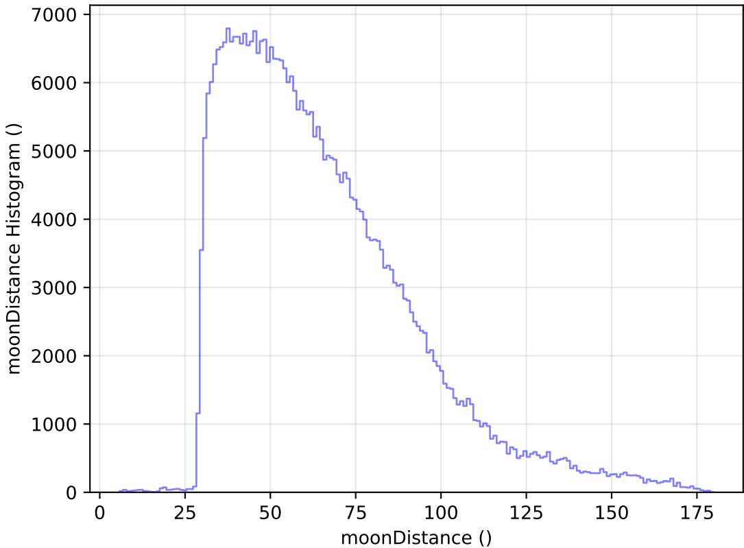
too_ignore_10_4v3.4_10yrs All sky y band: moonDistance Histogram
