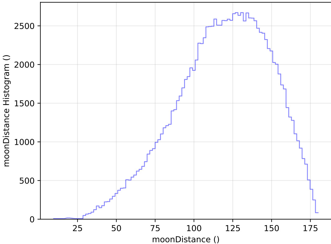
too_ignore_10_4v3.4_10yrs All sky u band: moonDistance Histogram
