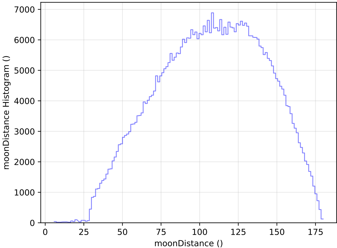
too_ignore_10_4v3.4_10yrs All sky r band: moonDistance Histogram
