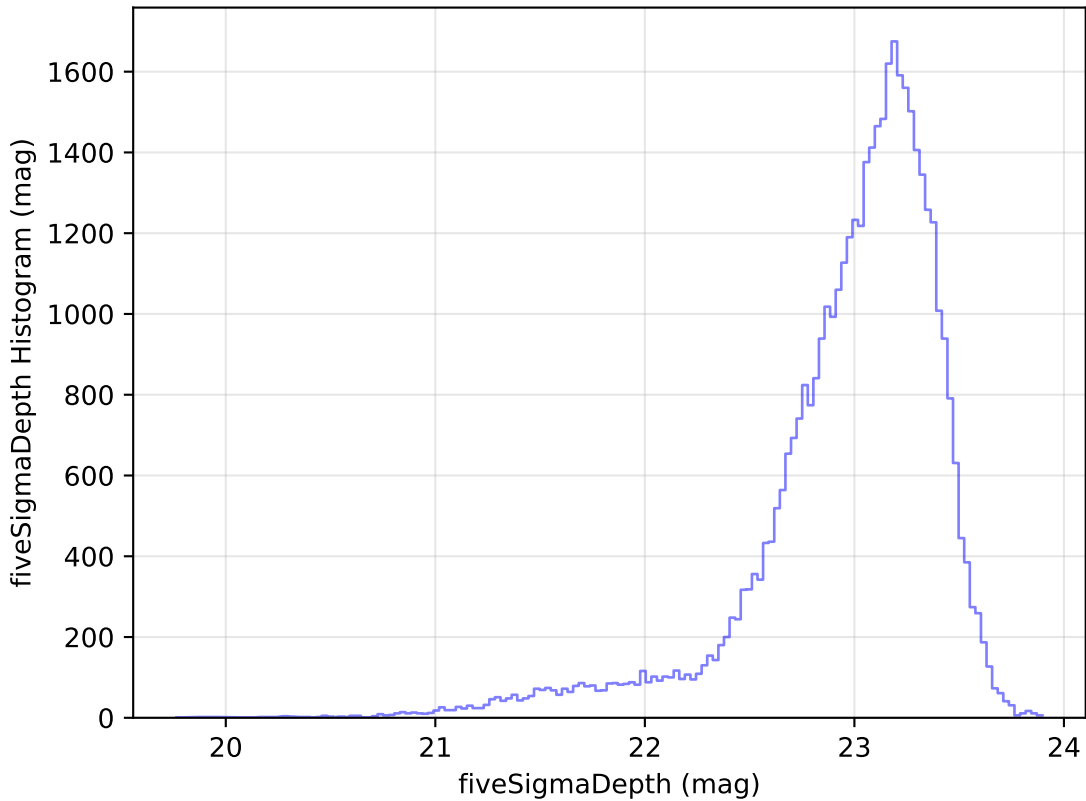
too_ignore_10_4v3.4_10yrs Yr 1 z band: fiveSigmaDepth Histogram
