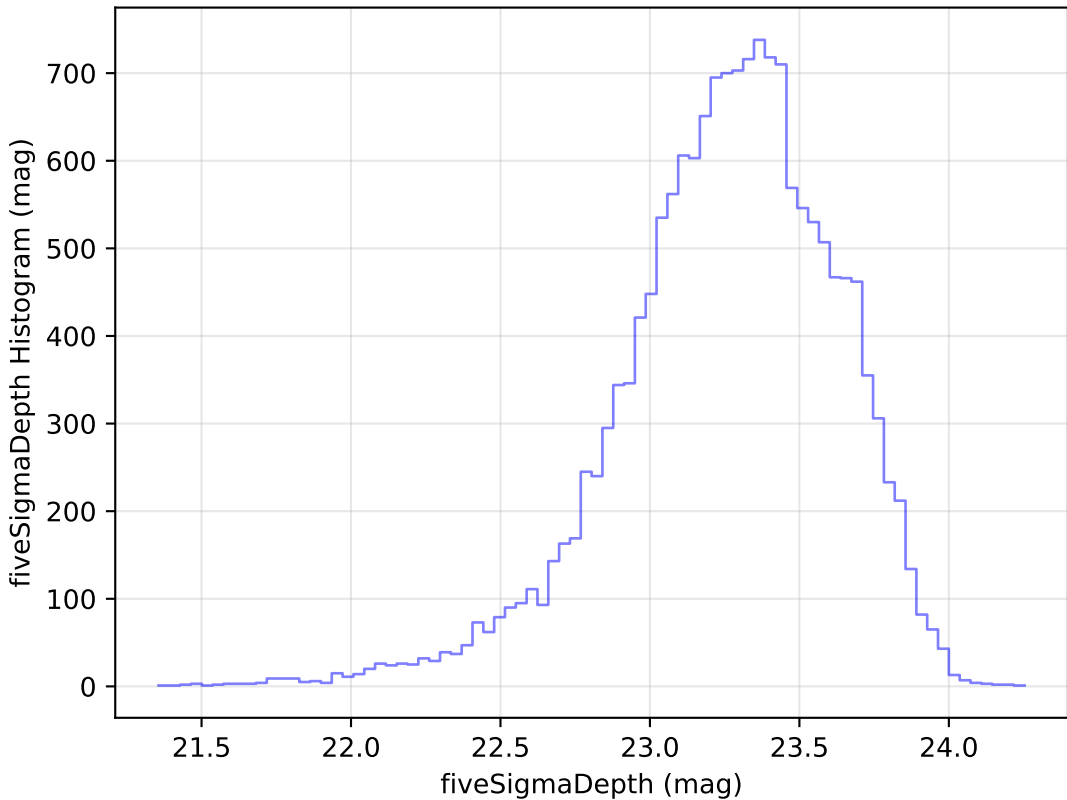
too_ignore_10_4v3.4_10yrs Yr 1 u band: fiveSigmaDepth Histogram
