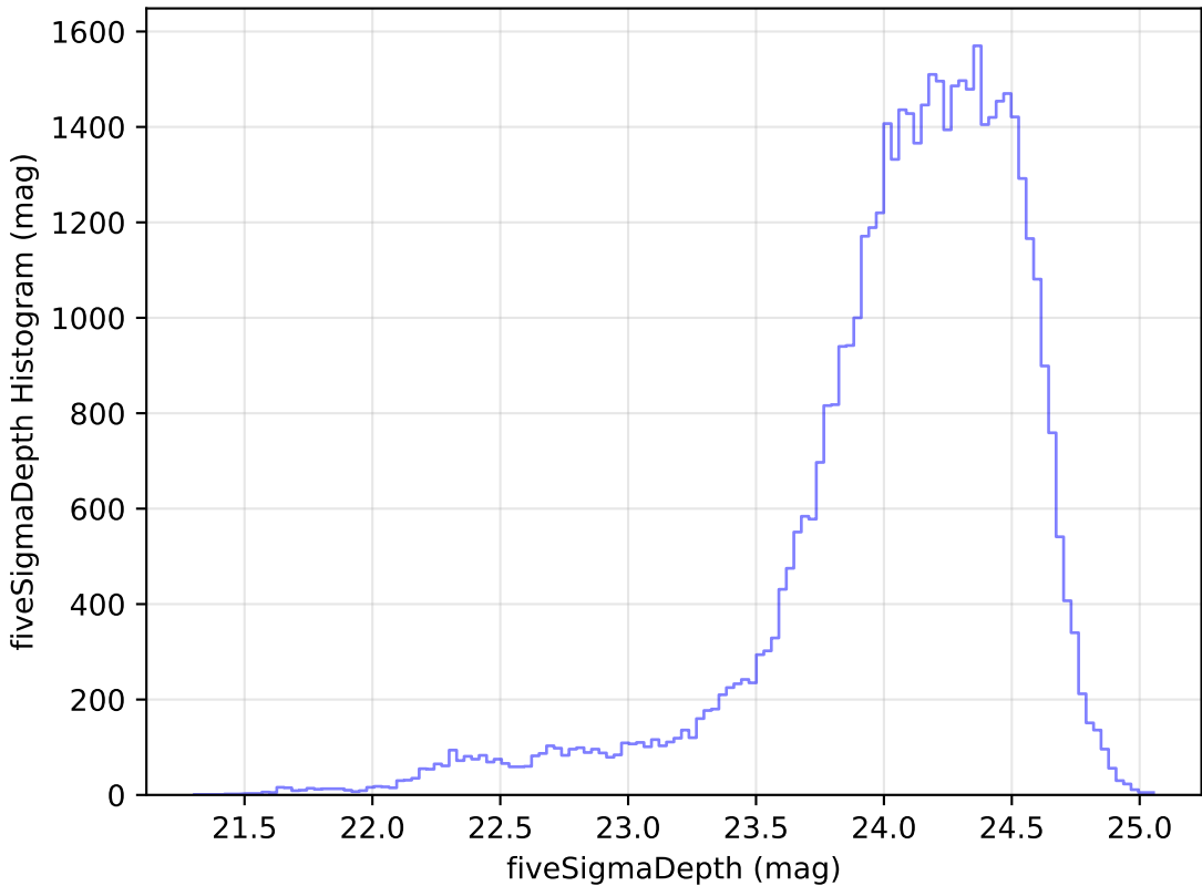
too_ignore_10_4v3.4_10yrs Yr 1 r band: fiveSigmaDepth Histogram
