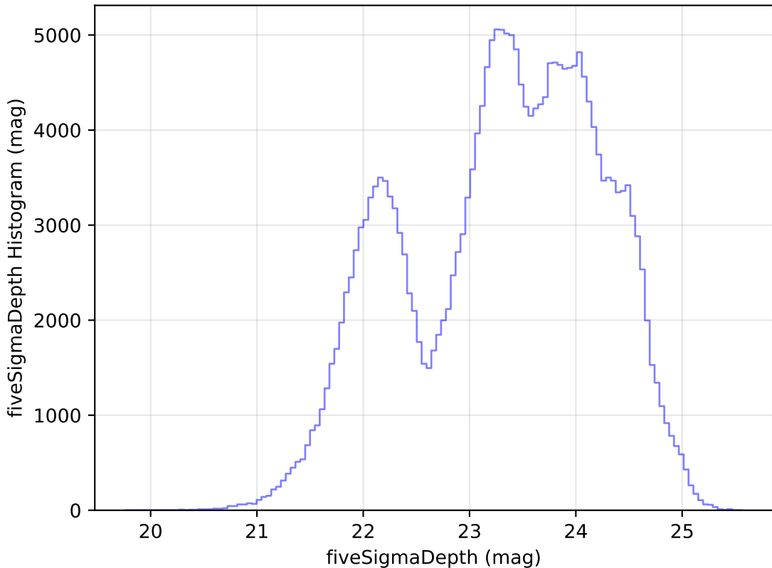
too_ignore_10_4v3.4_10yrs Yr 1 all bands: fiveSigmaDepth Histogram
