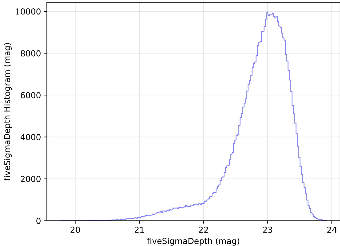
too_ignore_10_4v3.4_10yrs WFD z band: fiveSigmaDepth Histogram
