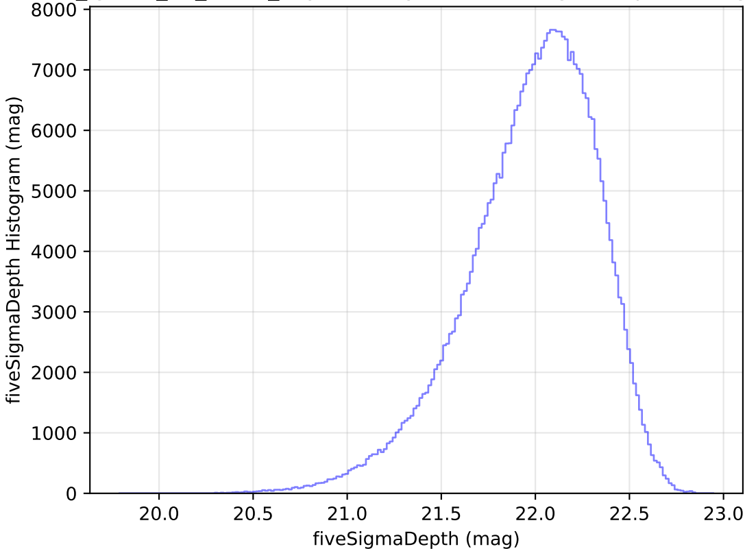
too_ignore_10_4v3.4_10yrs WFD y band: fiveSigmaDepth Histogram
