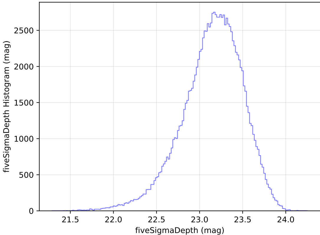
too_ignore_10_4v3.4_10yrs WFD u band: fiveSigmaDepth Histogram
