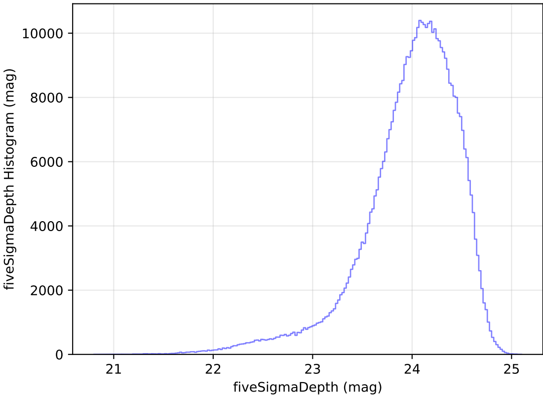
too_ignore_10_4v3.4_10yrs WFD r band: fiveSigmaDepth Histogram
