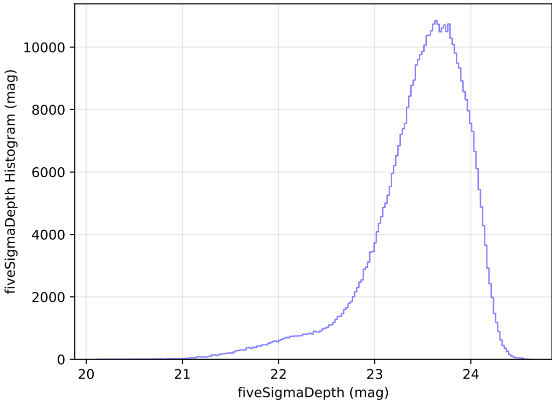
too_ignore_10_4v3.4_10yrs WFD i band: fiveSigmaDepth Histogram
