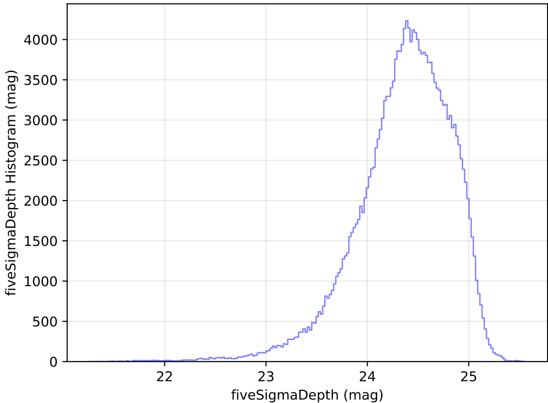
too_ignore_10_4v3.4_10yrs WFD g band: fiveSigmaDepth Histogram
