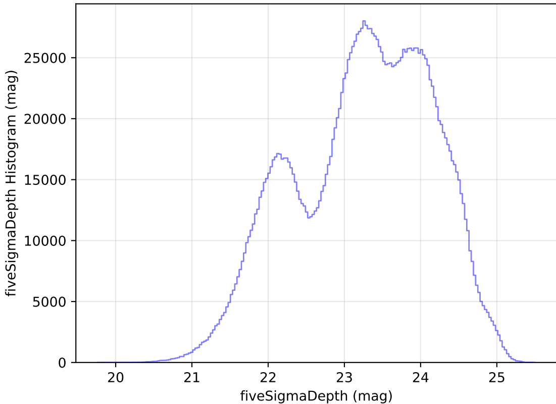
too_ignore_10_4v3.4_10yrs WFD all bands: fiveSigmaDepth Histogram
