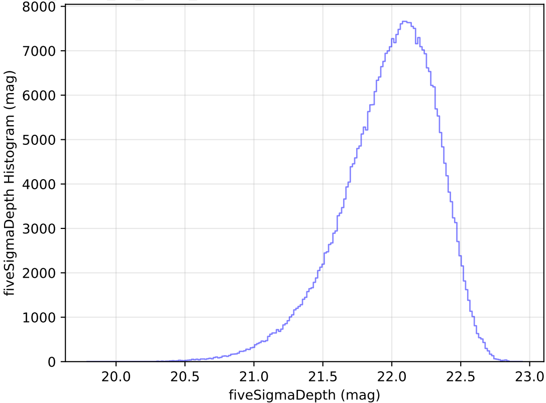
too_ignore_10_4v3.4_10yrs All sky y band: fiveSigmaDepth Histogram
