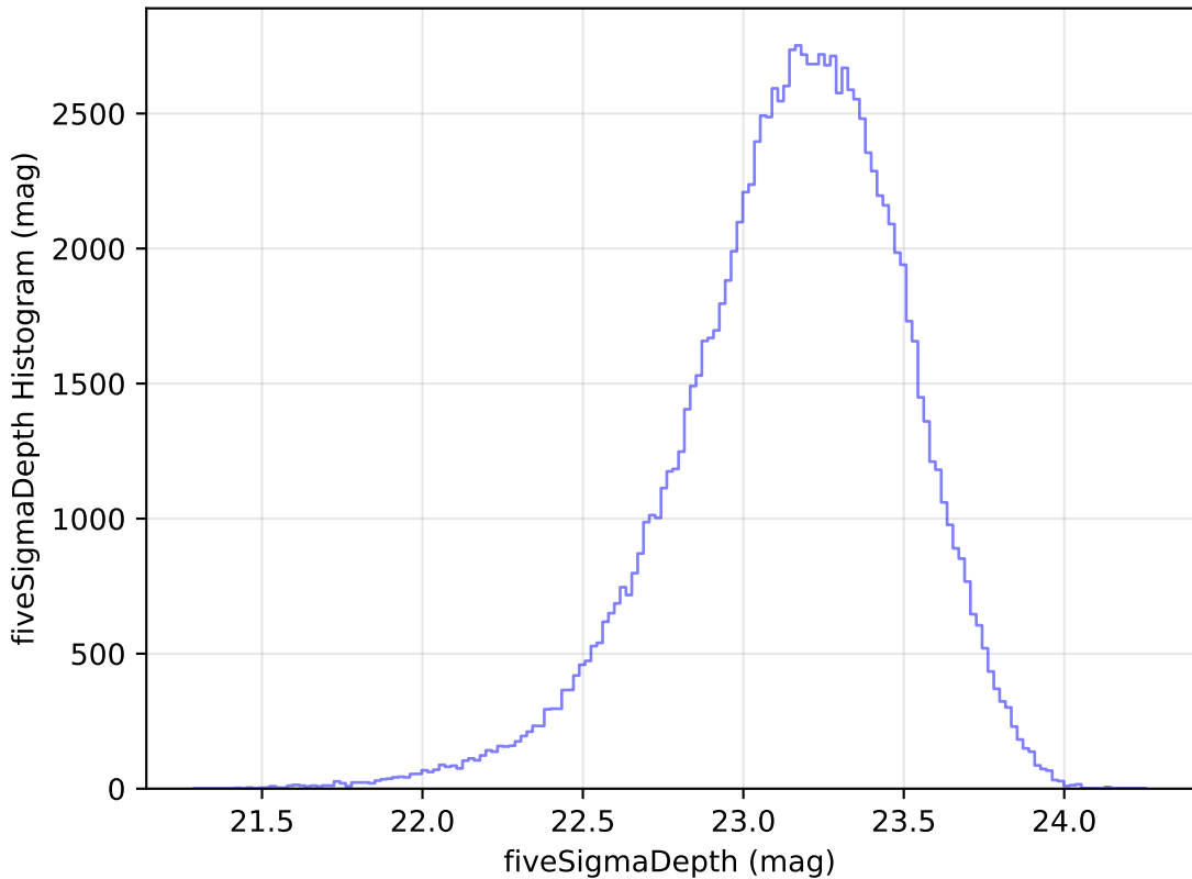
too_ignore_10_4v3.4_10yrs All sky u band: fiveSigmaDepth Histogram
