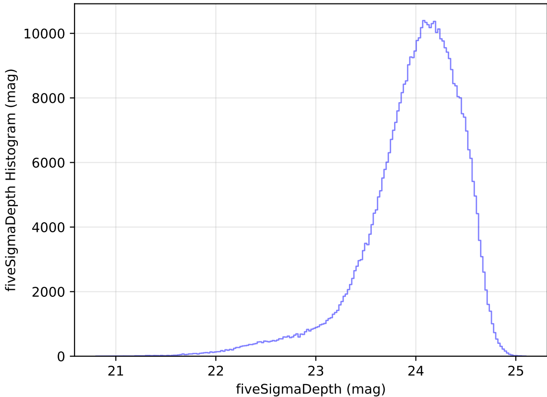
too_ignore_10_4v3.4_10yrs All sky r band: fiveSigmaDepth Histogram
