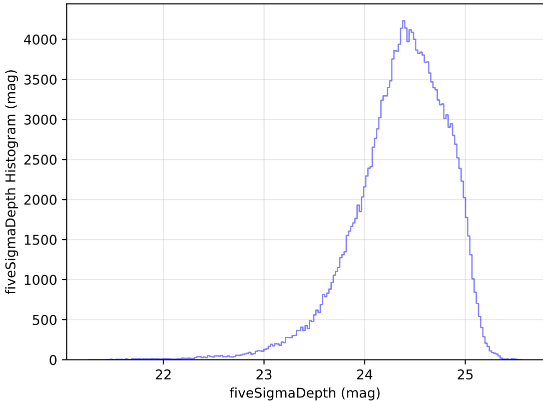
too_ignore_10_4v3.4_10yrs All sky g band: fiveSigmaDepth Histogram
