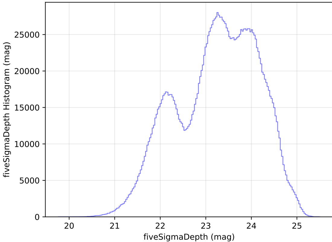
too_ignore_10_4v3.4_10yrs All sky all bands: fiveSigmaDepth Histogram
