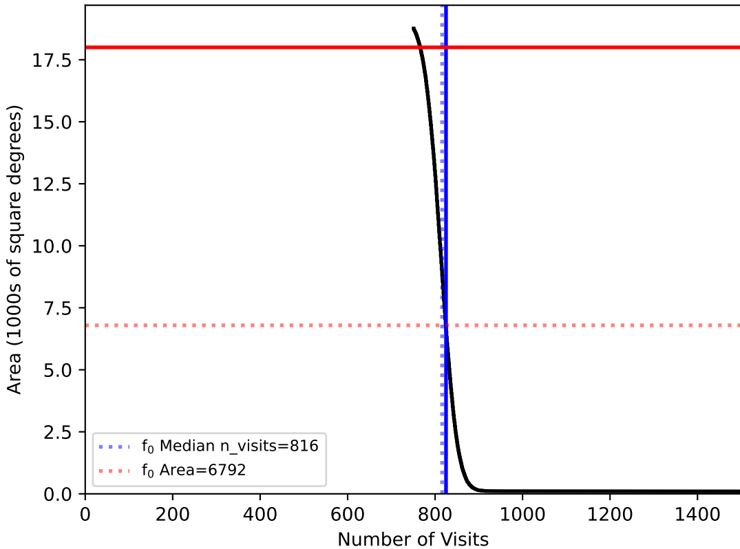
too_ignore_10_4v3.4_10yrs WFD: f0
