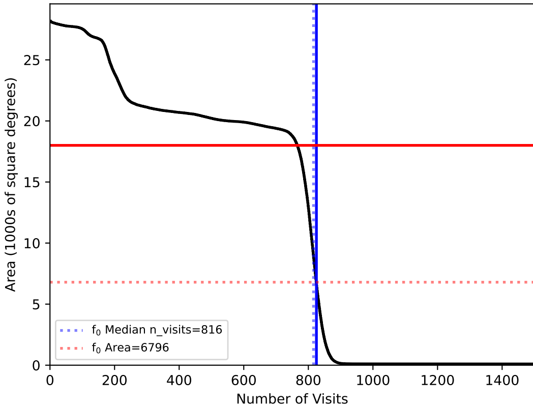
too_ignore_10_4v3.4_10yrs All sky: f0
