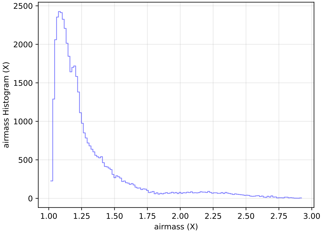
too_ignore_10_4v3.4_10yrs Yr 1 z band: airmass Histogram
