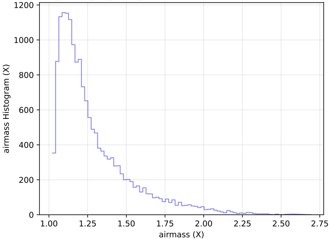
too_ignore_10_4v3.4_10yrs Yr 1 u band: airmass Histogram
