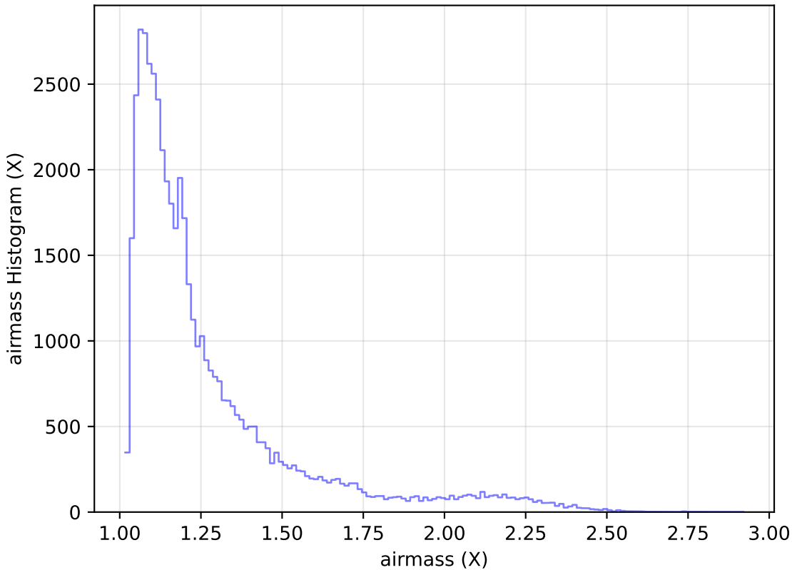
too_ignore_10_4v3.4_10yrs Yr 1 r band: airmass Histogram
