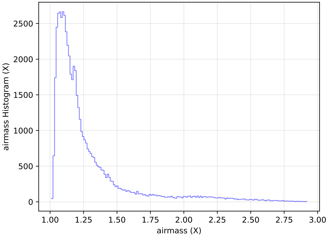
too_ignore_10_4v3.4_10yrs Yr 1 i band: airmass Histogram
