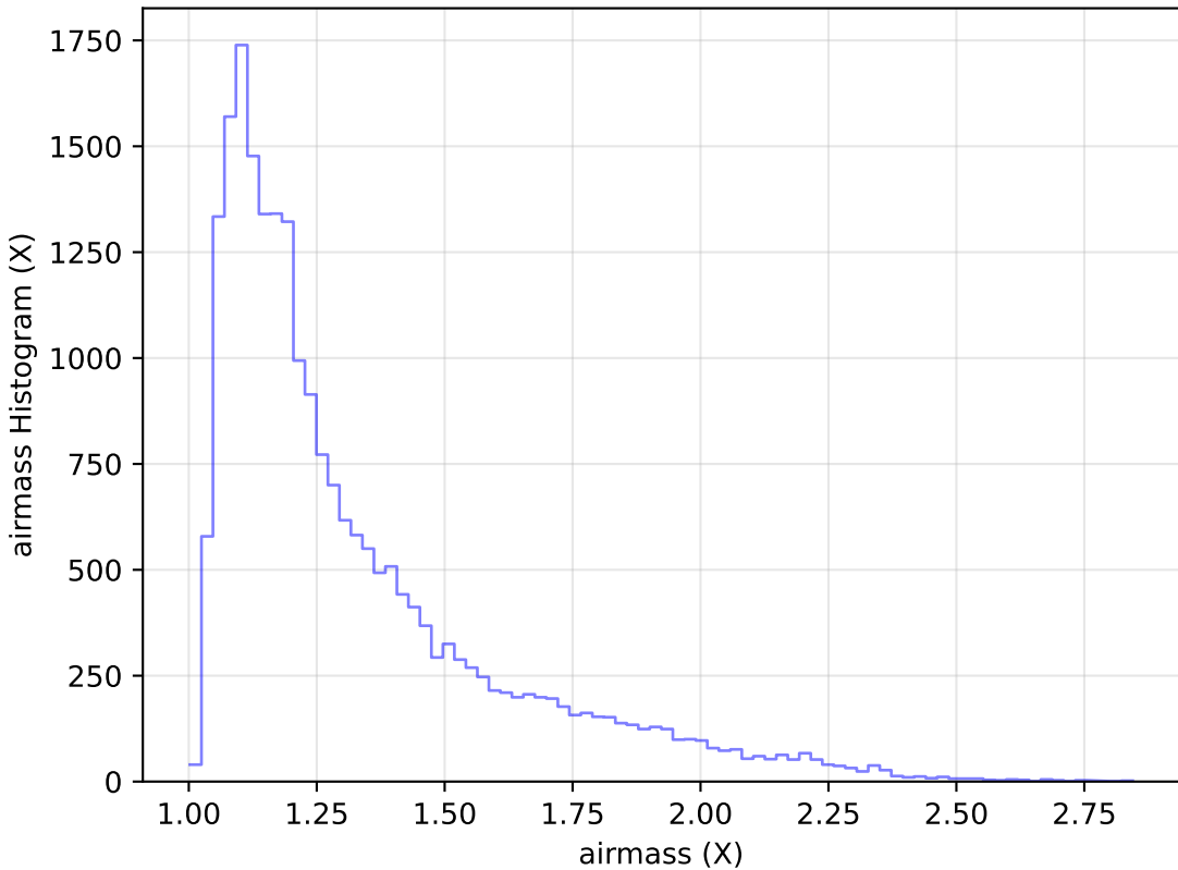
too_ignore_10_4v3.4_10yrs Yr 1 g band: airmass Histogram
