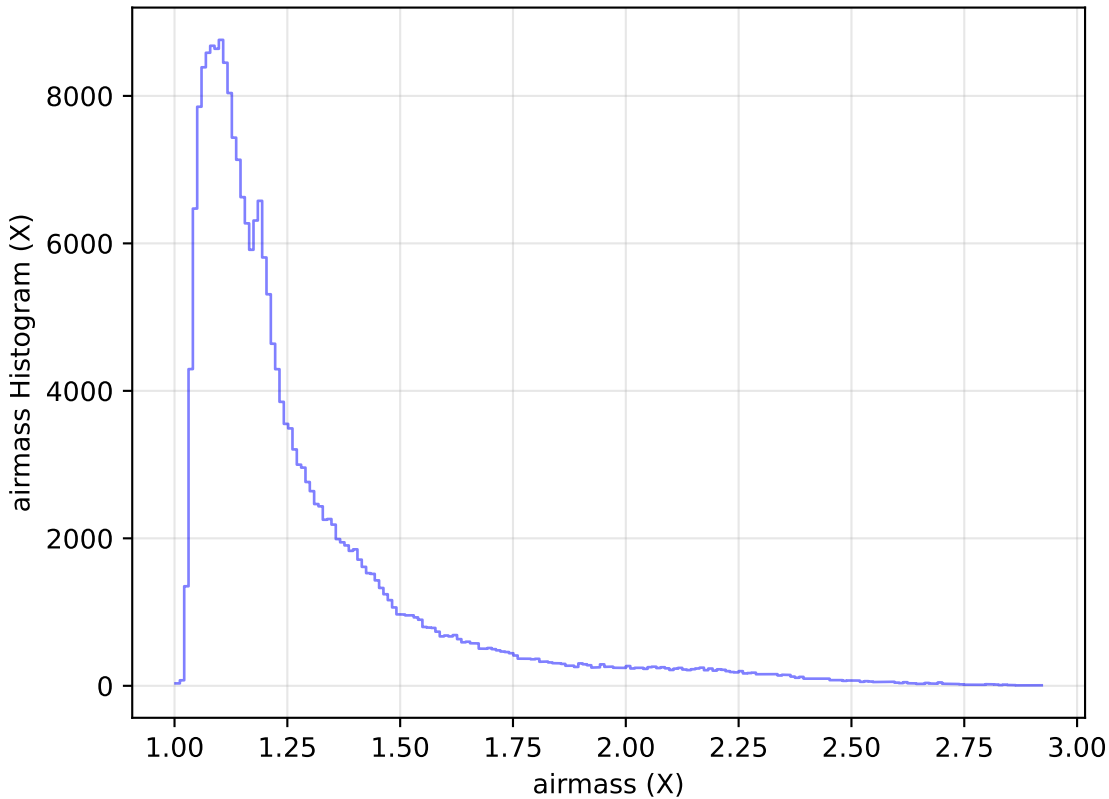
too_ignore_10_4v3.4_10yrs Yr 1 all bands: airmass Histogram
