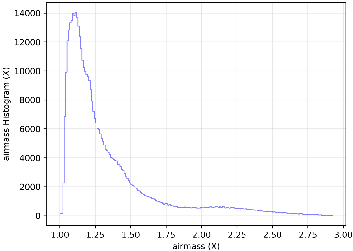
too_ignore_10_4v3.4_10yrs WFD z band: airmass Histogram
