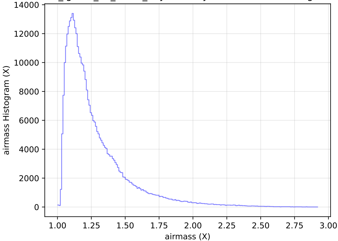
too_ignore_10_4v3.4_10yrs WFD y band: airmass Histogram
