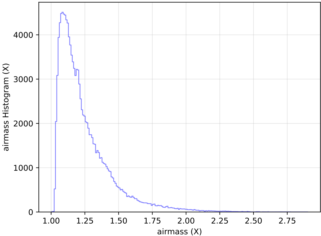
too_ignore_10_4v3.4_10yrs WFD u band: airmass Histogram
