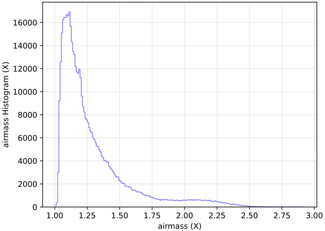
too_ignore_10_4v3.4_10yrs WFD r band: airmass Histogram
