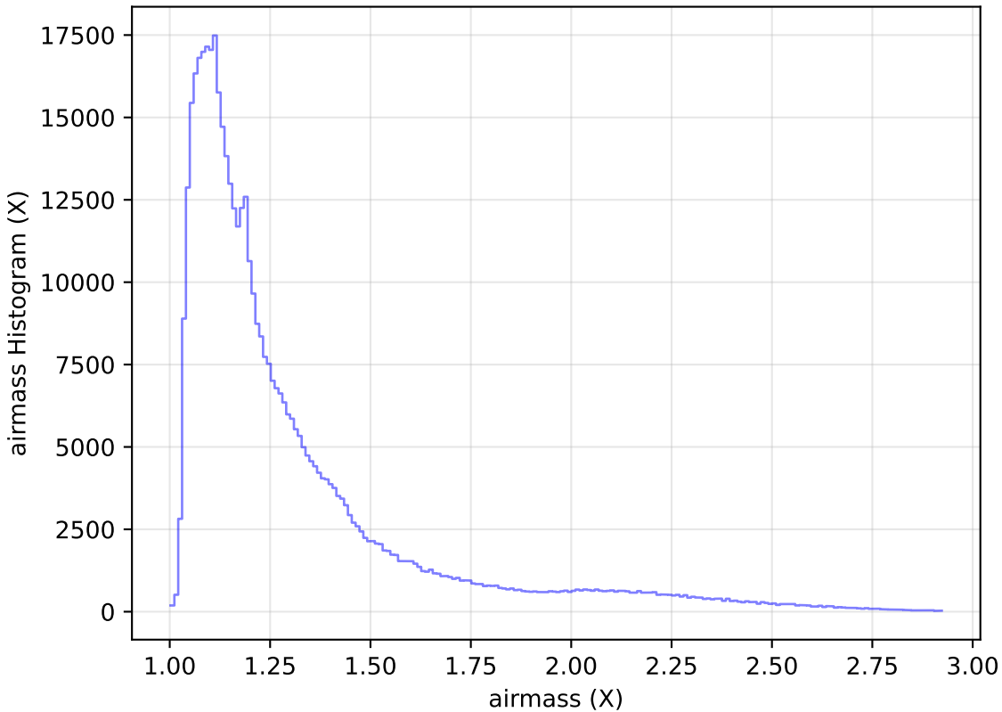
too_ignore_10_4v3.4_10yrs WFD i band: airmass Histogram
