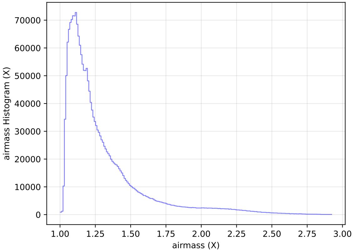
too_ignore_10_4v3.4_10yrs WFD all bands: airmass Histogram
