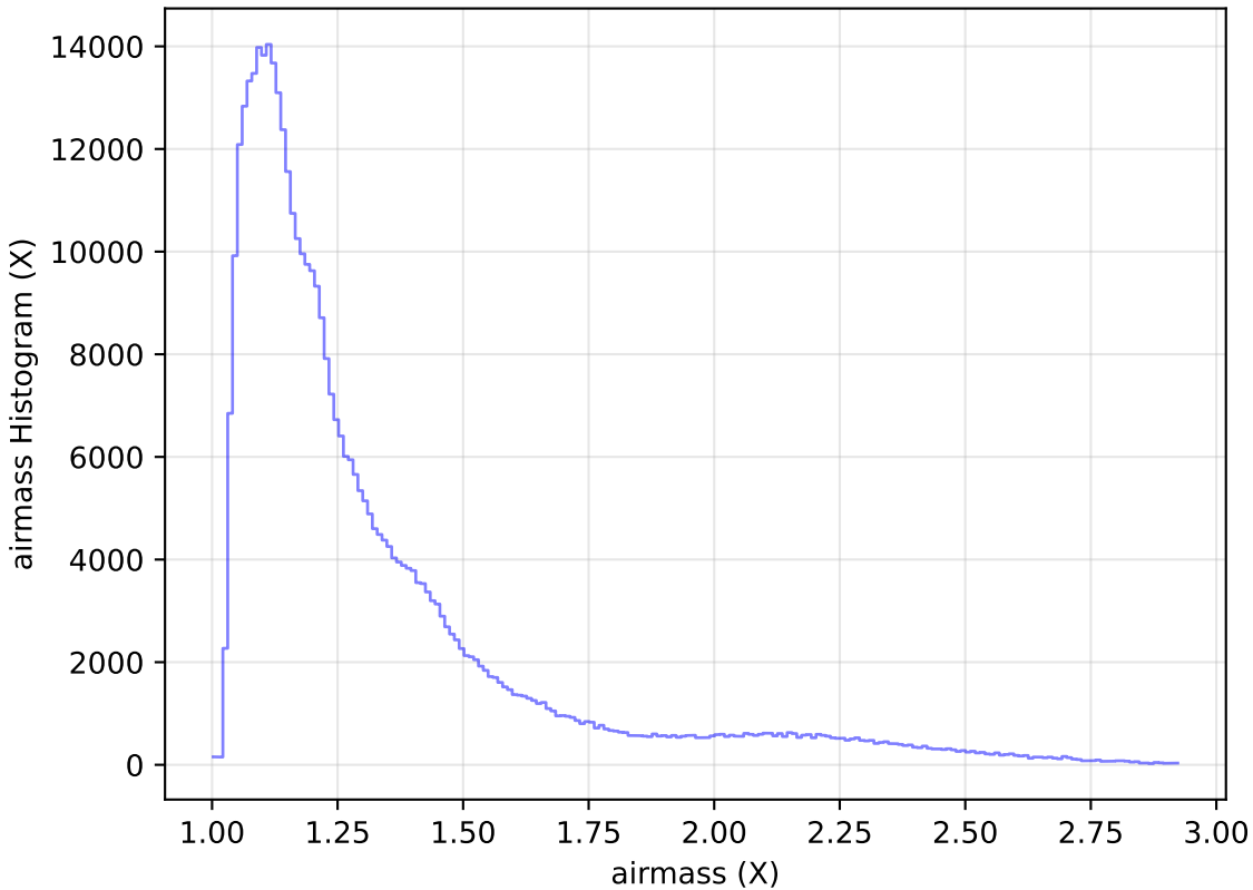
too_ignore_10_4v3.4_10yrs All sky z band: airmass Histogram
