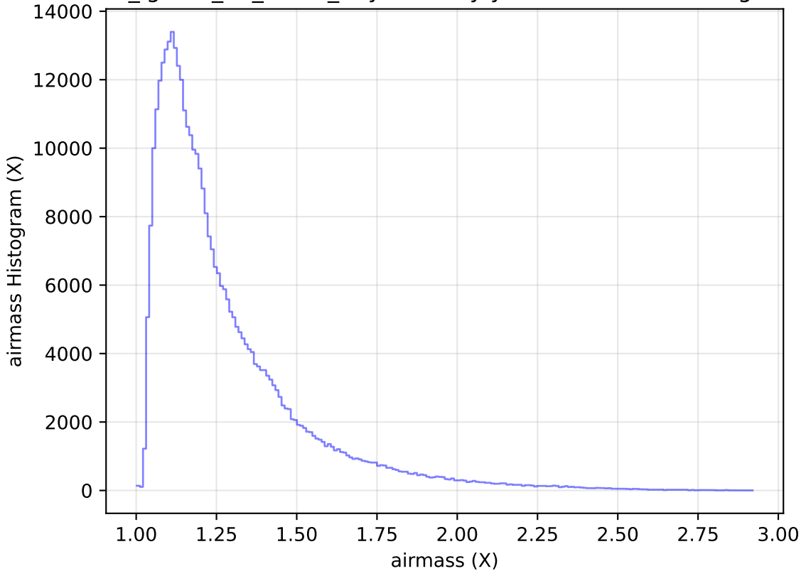
too_ignore_10_4v3.4_10yrs All sky y band: airmass Histogram
