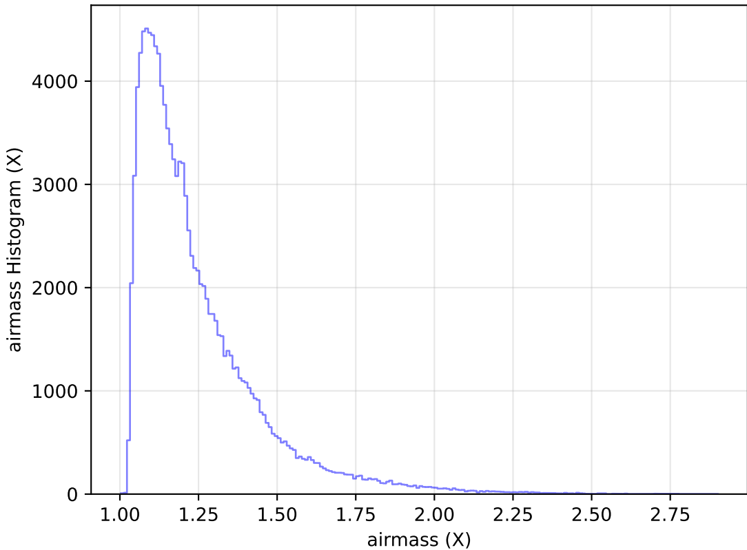
too_ignore_10_4v3.4_10yrs All sky u band: airmass Histogram
