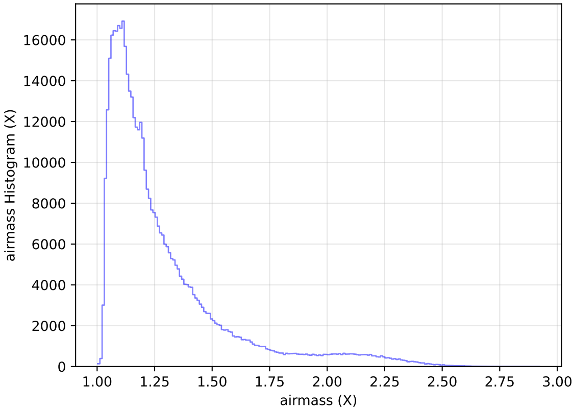
too_ignore_10_4v3.4_10yrs All sky r band: airmass Histogram
