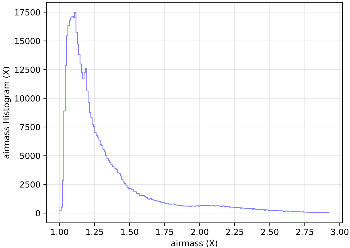
too_ignore_10_4v3.4_10yrs All sky i band: airmass Histogram
