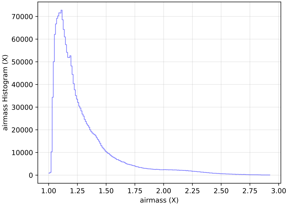
too_ignore_10_4v3.4_10yrs All sky all bands: airmass Histogram
