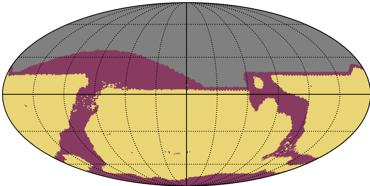
too_ignore_10_4v3.4_10yrs All sky: RapidRevisits
