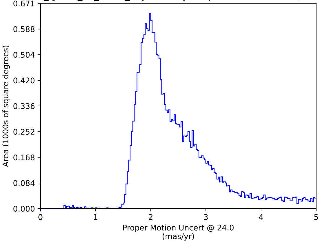
too_ignore_10_4v3.4_10yrs All sky: Proper Motion Uncert @ 24.0
