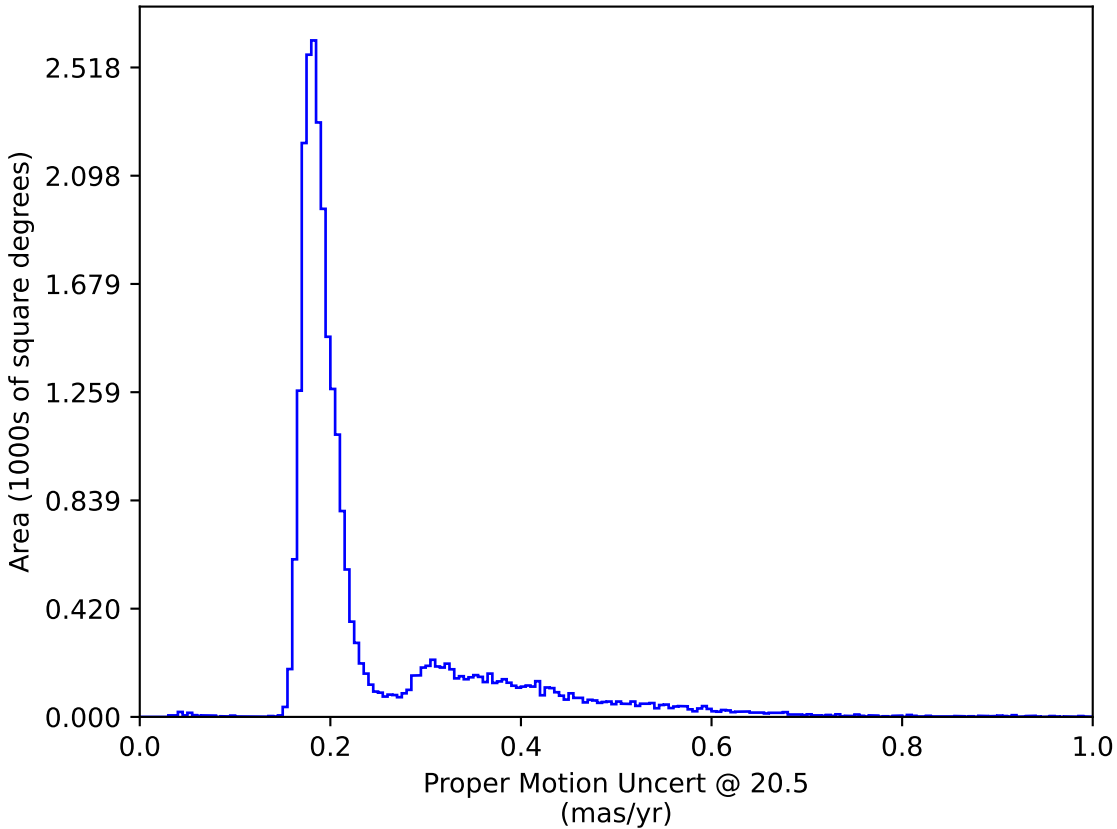
too_ignore_10_4v3.4_10yrs All sky: Proper Motion Uncert @ 20.5
