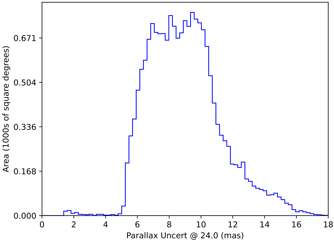
too_ignore_10_4v3.4_10yrs WFD: Parallax Uncert @ 24.0
