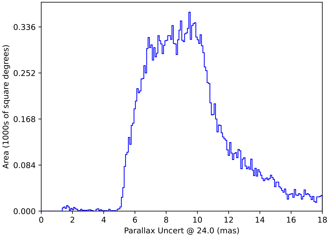
too_ignore_10_4v3.4_10yrs All sky: Parallax Uncert @ 24.0
