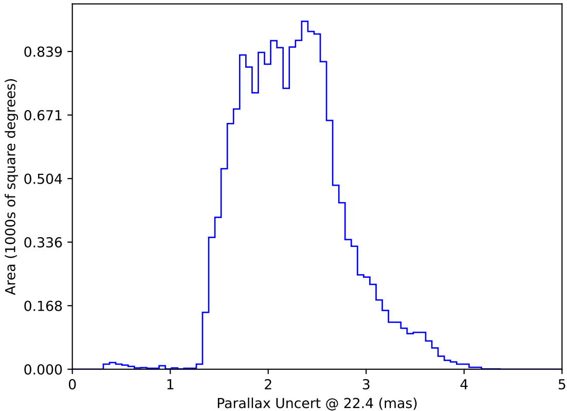
too_ignore_10_4v3.4_10yrs WFD: Parallax Uncert @ 22.4
