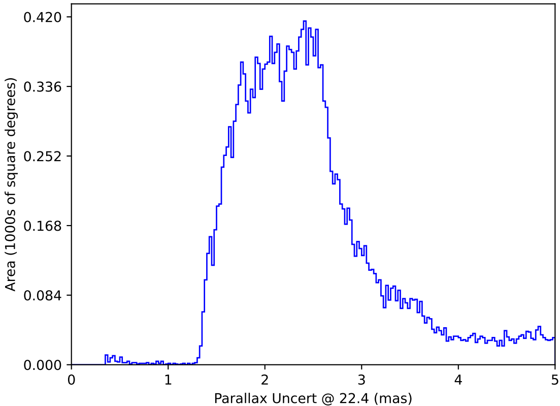
too_ignore_10_4v3.4_10yrs All sky: Parallax Uncert @ 22.4
