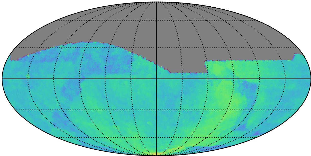
too_ignore_10_4v3.4_10yrs All sky: Parallax Coverage @ 24.0
