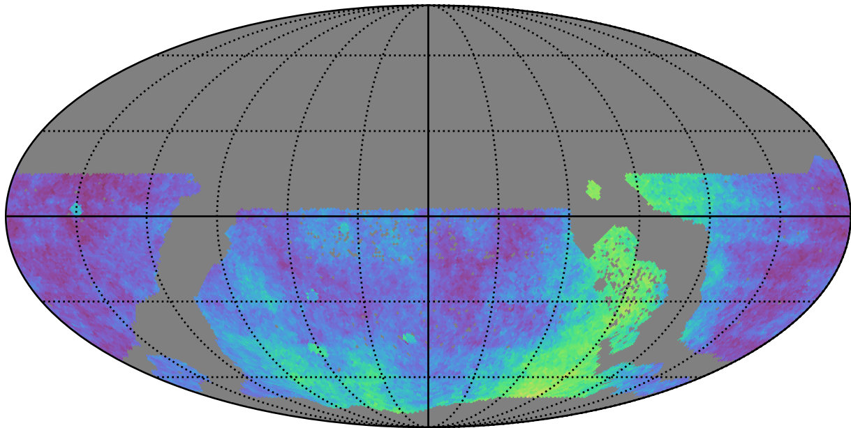
too_ignore_10_4v3.4_10yrs WFD: Parallax Coverage @ 22.4
