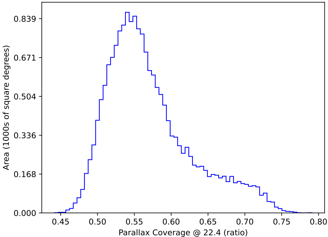
too_ignore_10_4v3.4_10yrs WFD: Parallax Coverage @ 22.4
