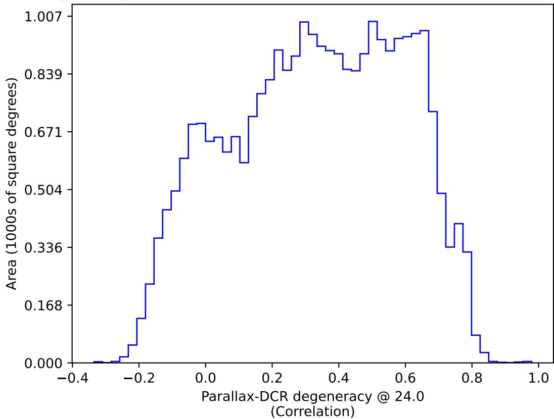
too_ignore_10_4v3.4_10yrs All sky: Parallax-DCR degeneracy @ 24.0
